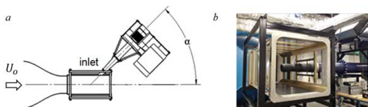
Figure 1. Inlet test facility having adjustable inlet angle \alpha , relative to the crosswind U_0 (a) and a picture of the installed inlet in the crosswind test section.
