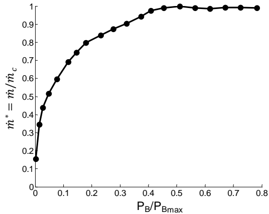
Figure 3. Inlet mass flow rate \dot{m}^* with increasing blower power, in the absence of crosswind.
